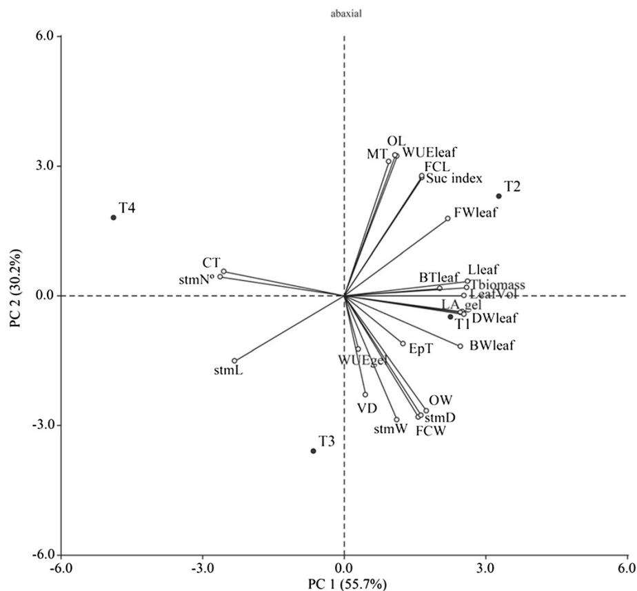
Figure 3 Principal component analysis showing the relationships between anatomy, morphology, and WUE in A. vera . T1 to T4, treatments; CT, cuticle thickness; stmN°, stomata number; stmL, stomata length; stmD, distance between stomata; stmW, stomata width; OW, ostiole width; OL, ostiole length; EpT, epidermis thickness; MT, mesophyll thickness; VD, distance between vascular bundles; FCW, photosynthetic cells width; FCL, photosynthetic cells length; BWleaf, leaf basal width; BTleaf, leaf basal thickness; LeafVol, leaf volume; LA, leaf area; FW, leaf fresh weight; Suc index, succulence index; DWleaf, leaf dry weight; Tbiomass, total biomass; WUE, water use efficiency.
